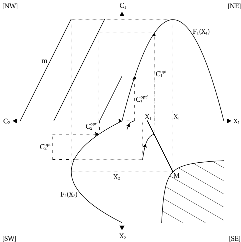
Figure 2: Perfect substitutes
